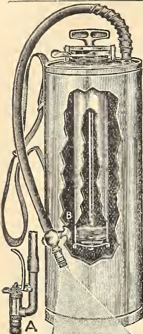
The reservoir holds 4 lbs. of Paris Green (or over a quart of powder). Is made in best manner, of tin, iron, steel and brass. We give this No. 2, larger and more powerful than No. 1, specially recommended for man can easily cover from 10 to 20 acres in one day. Price, $16.00.
